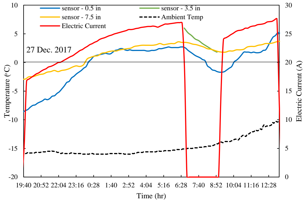
Figure 9. Electric current and temperature variations in different layers of the pavement and ambient temperature on 27 December 2017
