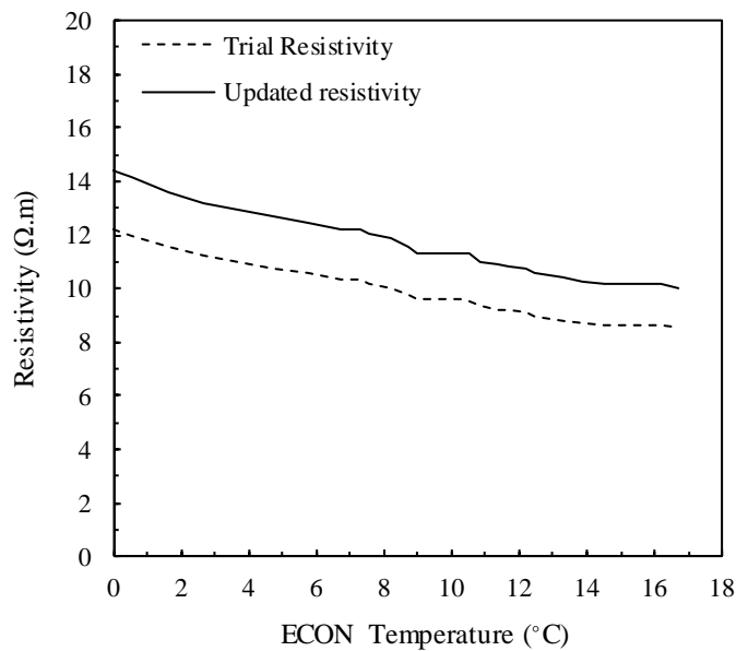
Figure 15. Electrical resistivity of ECON versus its temperature before and after model-updating using measured power demand of ECON HPS
