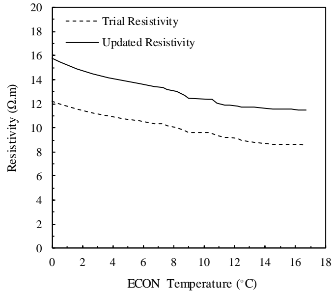
Figure 10. Electrical resistivity of ECON versus temperature for the FE model before and after model-updating by measured temperatures
