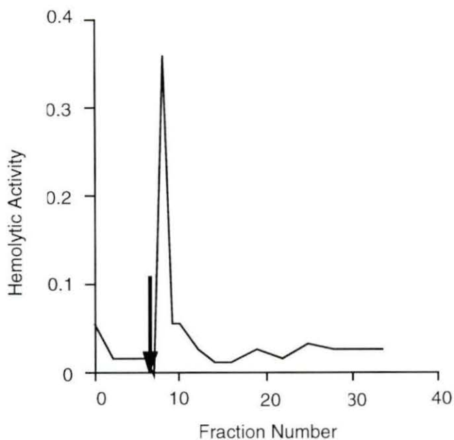
Figure 6. Profile of hemolytic activity from Sephadex G-200 column. Concentrated sHL supernatant was separated on a Sephadex G-200 column, and the fractions analyzed for hemolytic activity using the standard hemolytic assay. The arrow indicates the beginning of the void volume. Results are from a typical gel filtration experiment.
