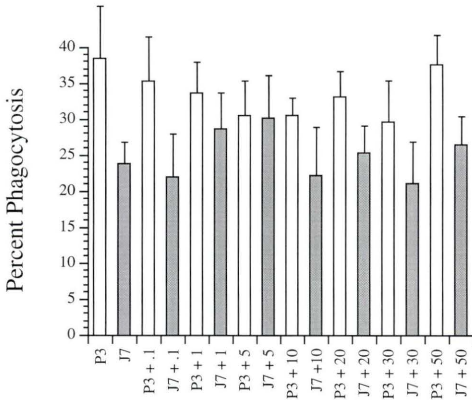
Figure 13. Effect of pHL on phagocytic activity of J774.A1 and P388.D1 cell lines. Numbers represent µg of pHL. White bars are results with P388.D1 cells, gray bars are results with J774.A1 cells. Data represent means \pm standard error of three experiments, duplicates within each experiment.
