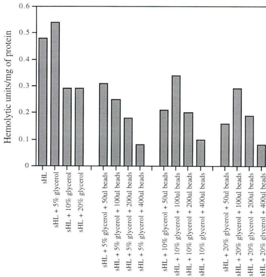
Figure 5. Effect of glycerol on the nonspecific adsorption of sHL to Sephacryl S-200 chromatography media. Increasing concentrations of glycerol (5, 10 or 20%) was added along with increasing amounts of Sephacryl S-200 beads to sHL containing fractions, incubated and the remaining HL activity assessed as described in the Materials and Methods. Data are from one experiment.
