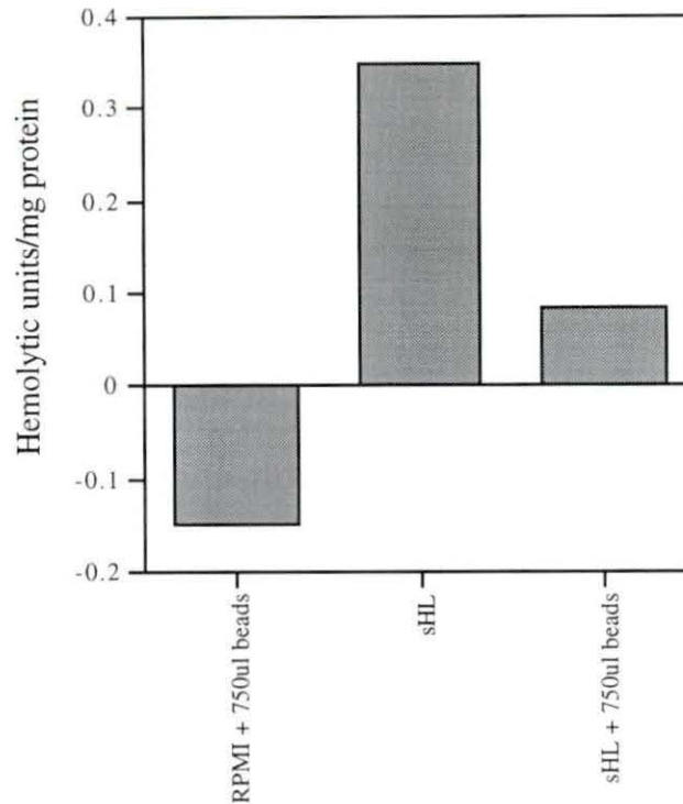
Figure 4. Effect of Sepharose beads on sHL activity. sHL containing fractions were mixed with Sepharose chromatography media and then examined for HL activity as described in the Materials and Methods. Data are from one experiment.
