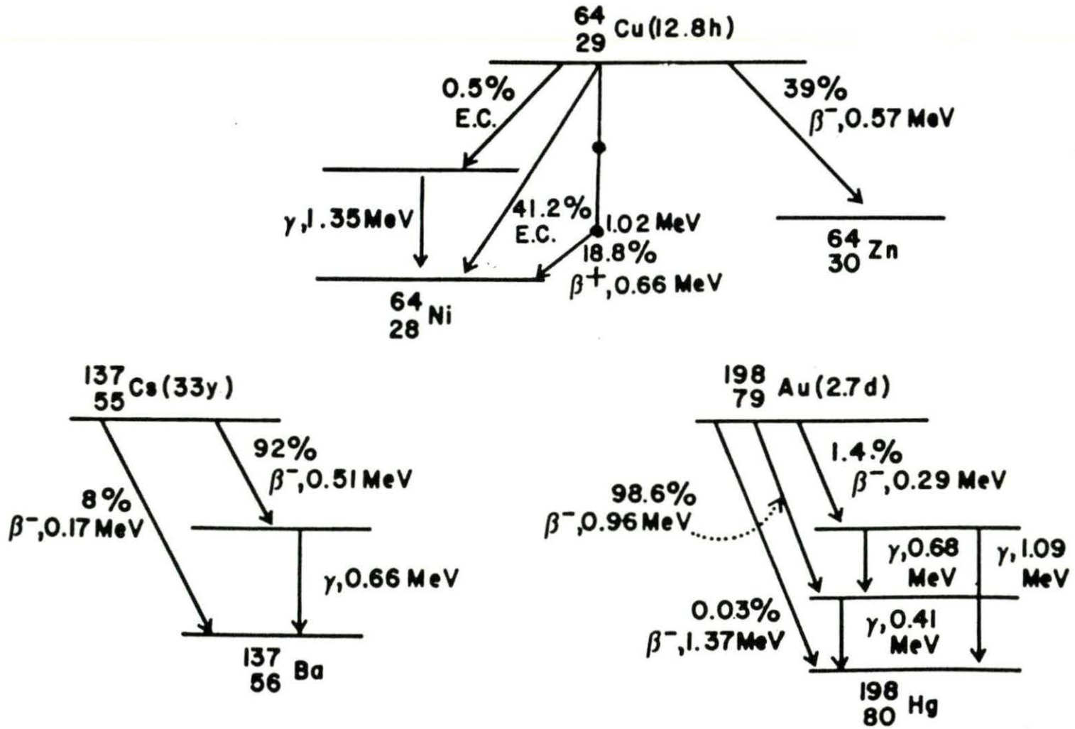
Fig. 3. Examples of radioisotope decay schemes
